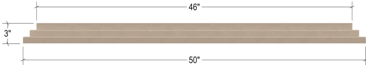
FRONT VIEW
