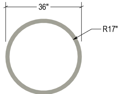
VP-CTS36S THICKNESS - 1"
