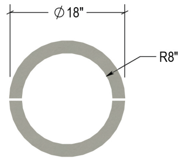
VP-CSB18S THICKNESS - 1"
