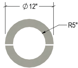
VP-CSB12S THICKNESS - 1"
