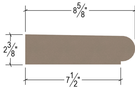
PROFILE VIEW
